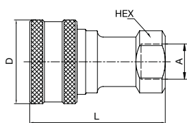
Female Thread
